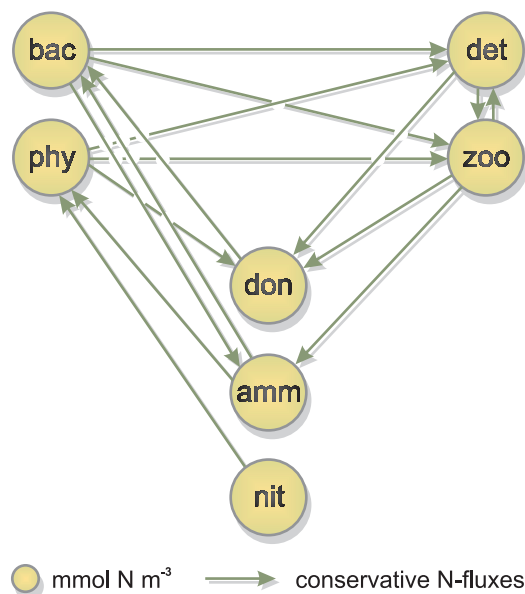
Figure 5: Structure of the Fasham et al. (1990) model with bacteria (bac), phytoplankton (phy), detritus (det), zooplankton (zoo), labile dissolved organic nitrogen (don), ammonium (amm) and nitrate (nit) as the seven state variables. The concentrations are in mmol N m -3 , all fluxes (green arrows) are conservative.
